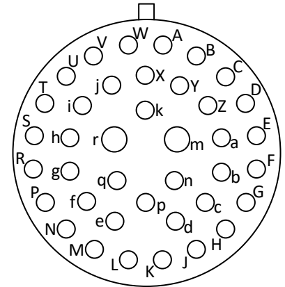
Female Solder Side
