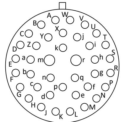
Male Solder Side
