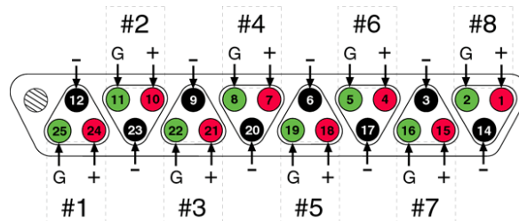
REAR VIEW OF MALE DB-25 CONNECTOR
